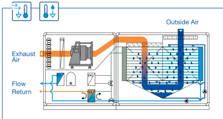
Fig. 3 The chiller operation scheme during “adiabatic” cycle [6]
