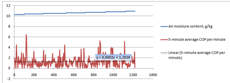
Fig. 6 Intake air moisture content and chiller's COP during operation within constant temperature
