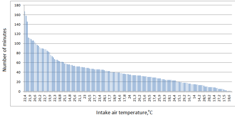
Fig. 4 Number of temperature – minutes during the 24th – 31st August, 2011
