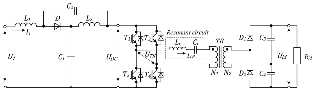
Fig. 1. General circuit diagram of the proposed converter.
