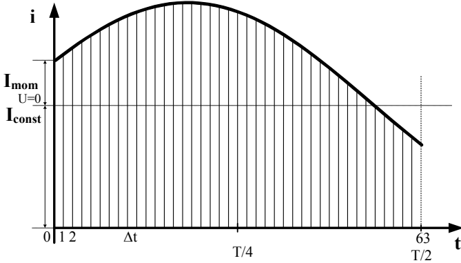
Fig. 8. Instant current calculation from measurements of Hall sensor.
