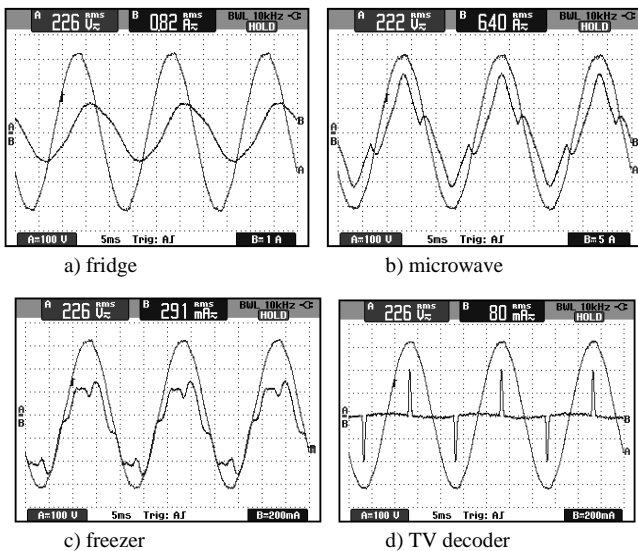
Fig. 5. Non-sinusoidal consumer waveform examples.
