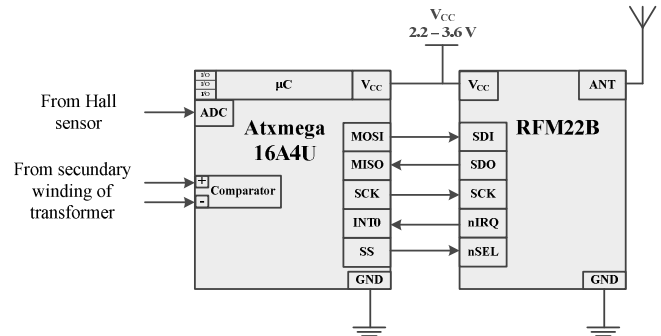
Fig. 10. Functional block and control of communication module.
