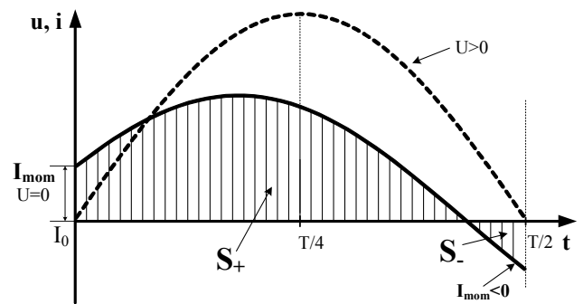
Fig. 7. The area ratio of the reactive nature of the consumer.
