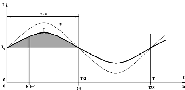
Fig. 9. Non-sinusoidal consumer waveform examples.
