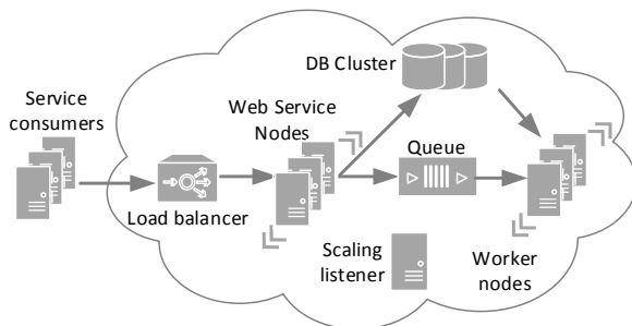
Fig. 1. High level architecture of the STORN.
