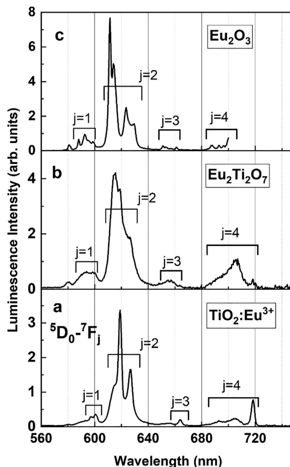
Fig. 8 – Luminescence spectra of TiO 2 :Eu 3+ nanoparticles (sample S2) (a), Eu 2 Ti 2 O 7 nanoparticles (sample S9) (b) and Eu 2 O 3 nanoparticles (c) under excitation of 7 F 0 - 5 D 2 transition in Eu 3+ .
