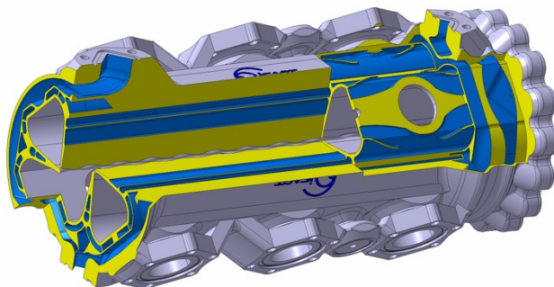
Figure 4: Improved iteration 3 RFQ.
