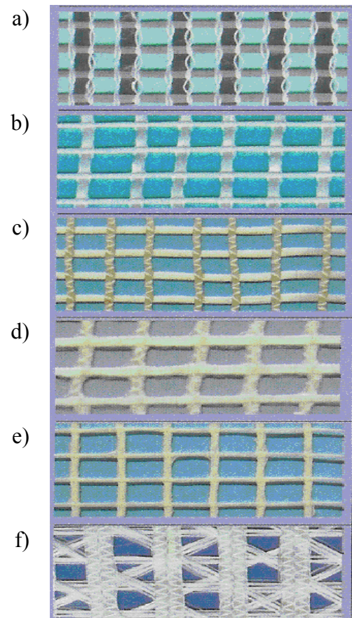
Figure 8. Fibre nets for concrete reinforcement (picture from [11])
