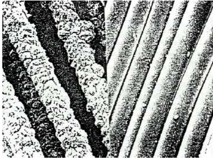
Figure 2. Surface of normal (left) glass fibers and AR fibers (right) after exposure to cement environment (picture from [1])
