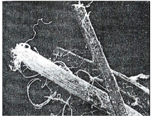
Figure 6. Specially developed polypropylene fibers with higher bond to cement and concrete matrix (picture from [7])
