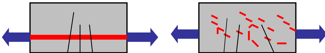
Figure 1. Long and short fibers reinforcement under tensile load in concrete (two different load bearing mechanisms)
