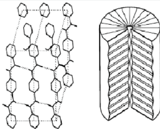
Figure 4. Aramid unit cell and fibre structure [5]
