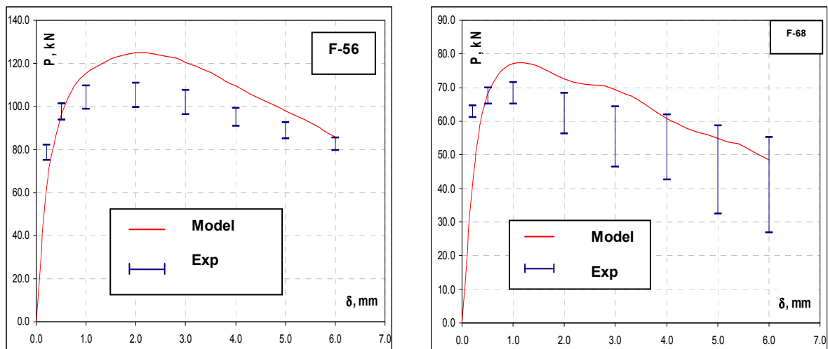
Fig. 4. SFRC prisms post-cracking behavior under 4 point bending. Mix F56 (left picture); mix F68 (right picture).
