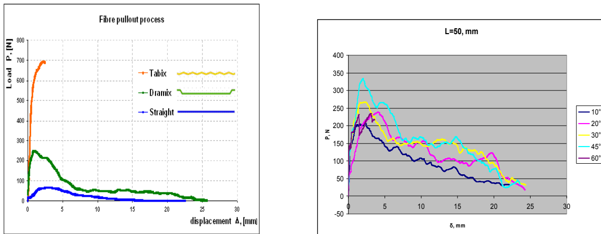
Fig.2. Pull-out low for different form fibers embedded at 25 mm having \alpha = 0^\circ (left picture); Dramix fibers (embedded at 25 mm) pull-out lows depending on \alpha = 0^\circ; 10^\circ; 20^\circ; 30^\circ; 45^\circ; 60^\circ
