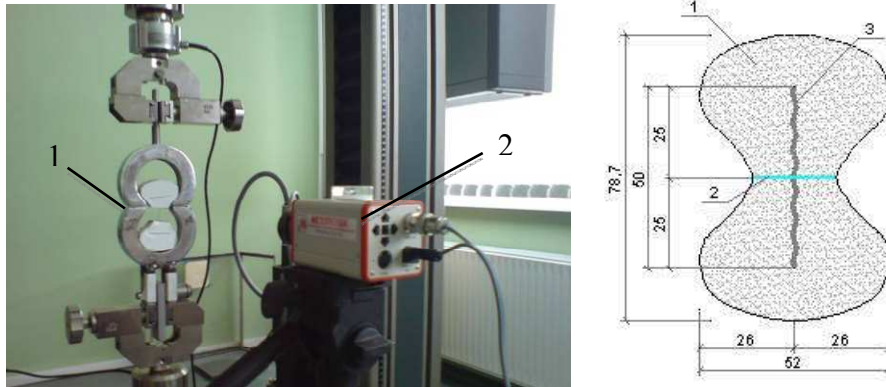
Fig.1. Fiber pull-out experimental set-up: 1-testing grips, 2-videoextensometer (Left picture); concrete sample with embedded fibre 1-concrete matrix, 2-plastic separator; 3-steel fiber.
