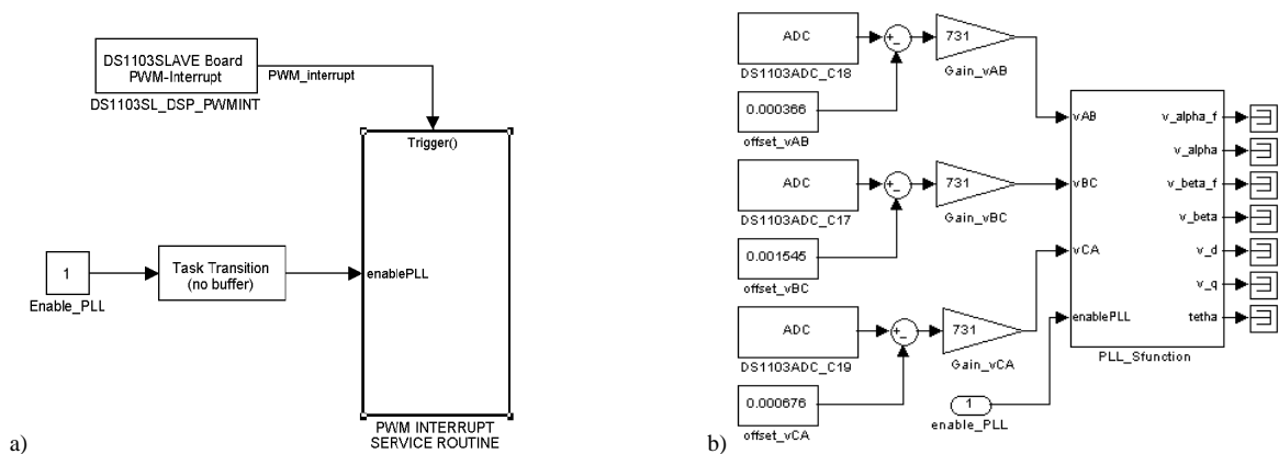
Fig.8. Matlab/Simulink implementation of the investigated system using DSPACE RTI tools: a) The main interrupt service routine block; b) PLL algorithm and the ADC task.
