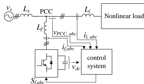
Fig.1. Parallel active power filter system.
