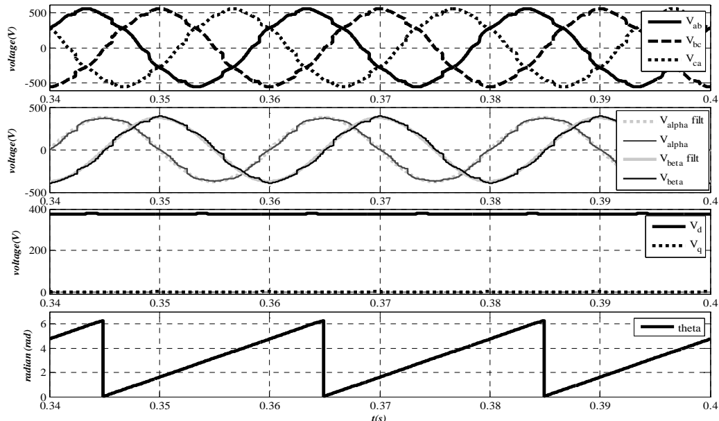
Fig.7. Simulated PLL characteristics with distorted voltage source – from top: PCC line voltages, voltage in the stationary \alpha\beta reference frame before and after the SSI filter, voltage in the synchronous dq reference frame and phase of the of the phasor of the fundamental component.
