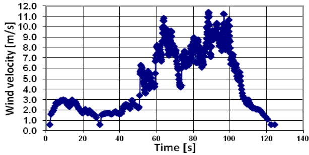
Fig. 1 Wind velocity pattern of moving freight train
