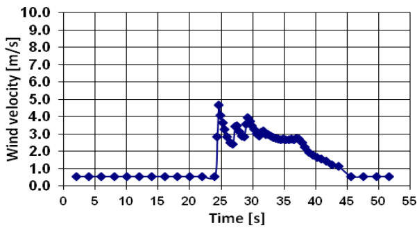
Fig. 2. Wind velocity pattern of moving electrical train.
