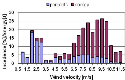
Fig. 4. Potential of energy generation from freight train wind pattern.
