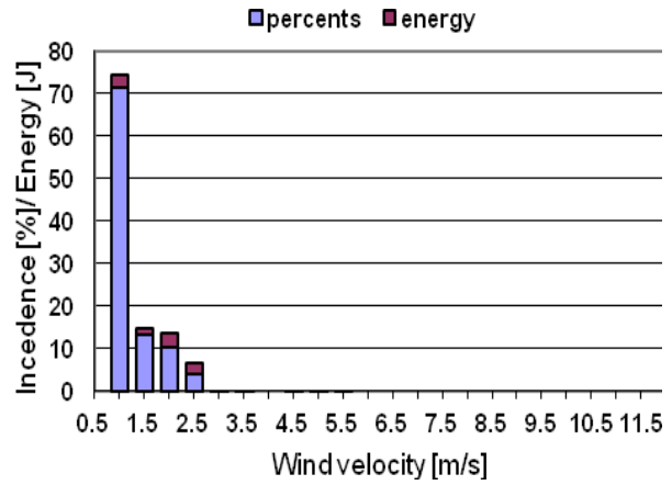
Fig. 5. Potential of energy generation from freight trucks wind pattern.
