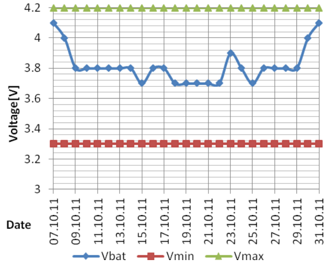
Fig. 7. Battery voltage change during the field test.
