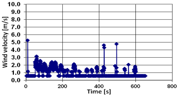
Fig. 3 Wind velocity pattern of moving freight trucks.
