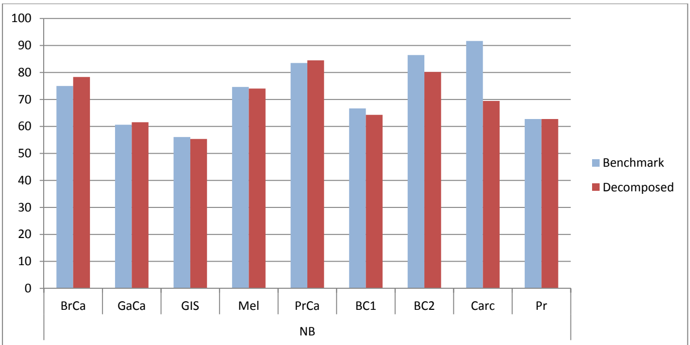
Fig. 1. Results of Naïve Bayes algorithm across all data sets
