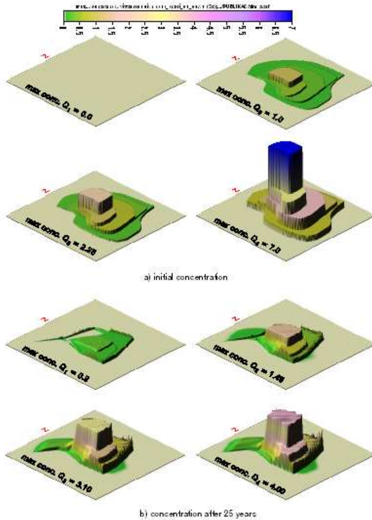
Fig. 5. Sanitation version A. Isometric images of chloride concentration [ \text{kg}/\text{m}^3 ] versus time
