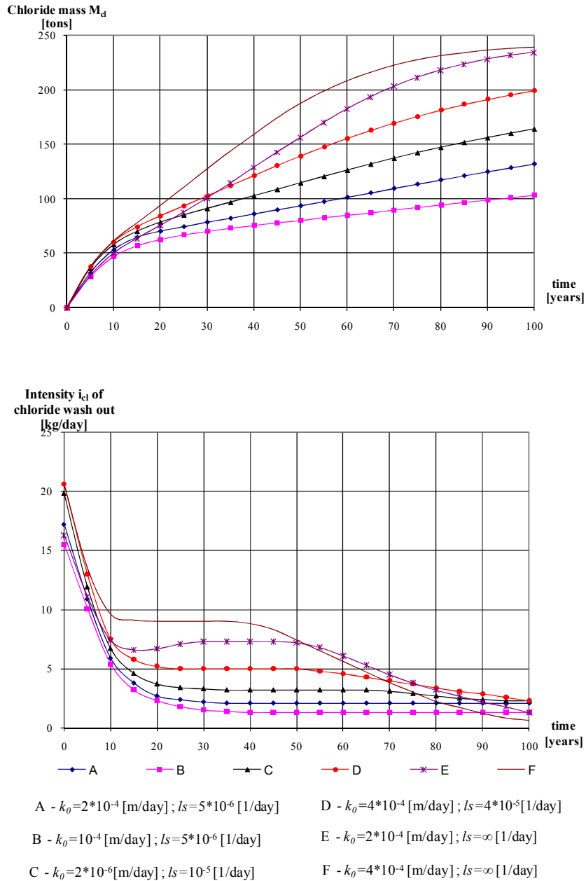
Fig. 4. Wash out of chlorides versus time for the sanitation versions A, B, C, D, E, F. After the first (10-15) years, the wash out gets slower, especially, for the versions A, B, C. In Table 5, the maximal concentration (in the zone 1, version A) is given versus time. Decrease of the concentration in the Q_4 layer is due to the assumption that the flow q_D is clean.
