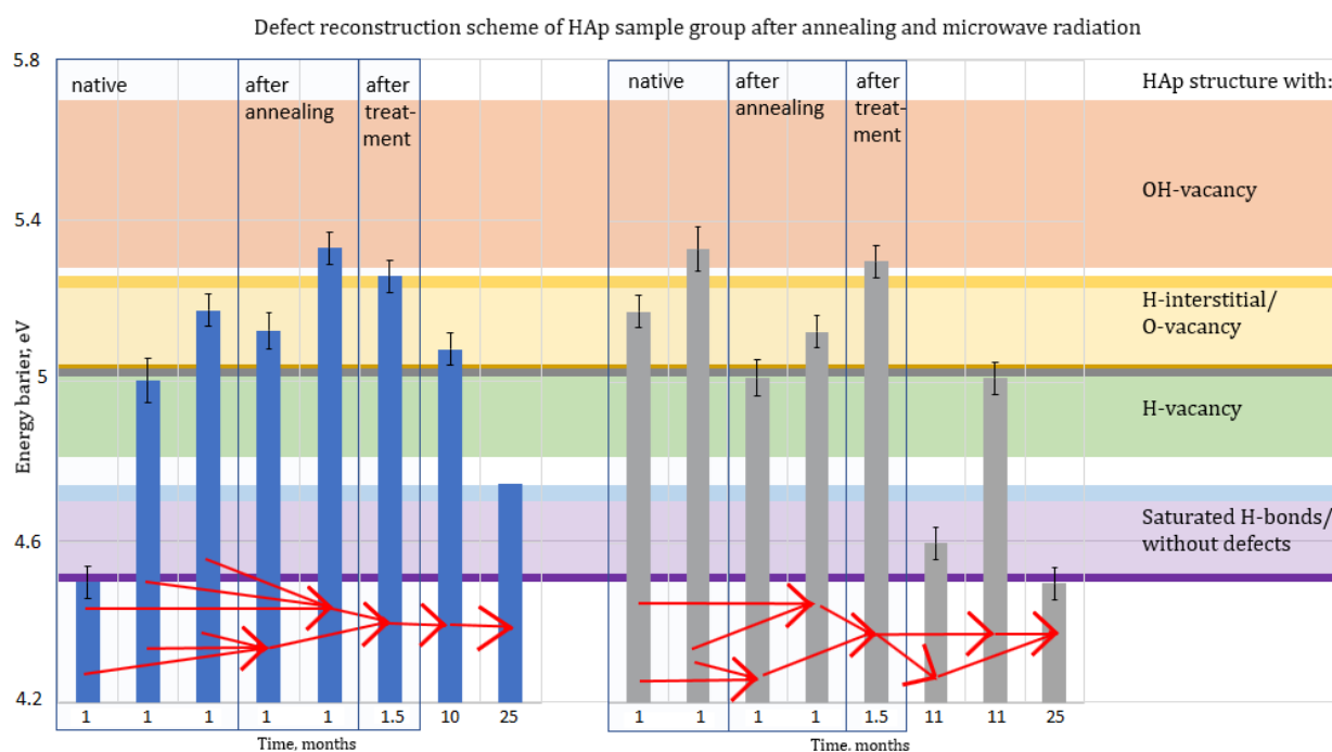
Fig. 3.15. Schemes of defect reconstructions in HAp after annealing and microwave irradiation.
