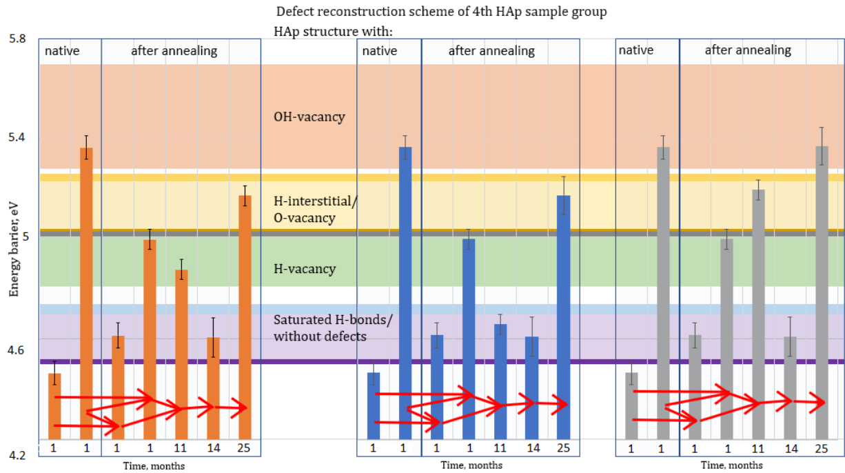
Fig. 3.9. Schemes of defect reconstructions in samples of the Group 4.
