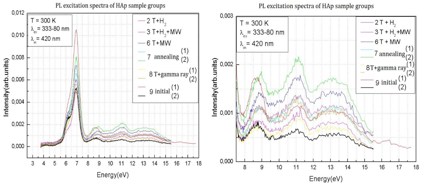
Fig. 3.18. PL excitation spectra at \lambda = 420 \text{ nm} : left – in the range of 3.5\text{--}18 \text{ eV} ; right – in the range of 7.5\text{--}18 \text{ eV} .
