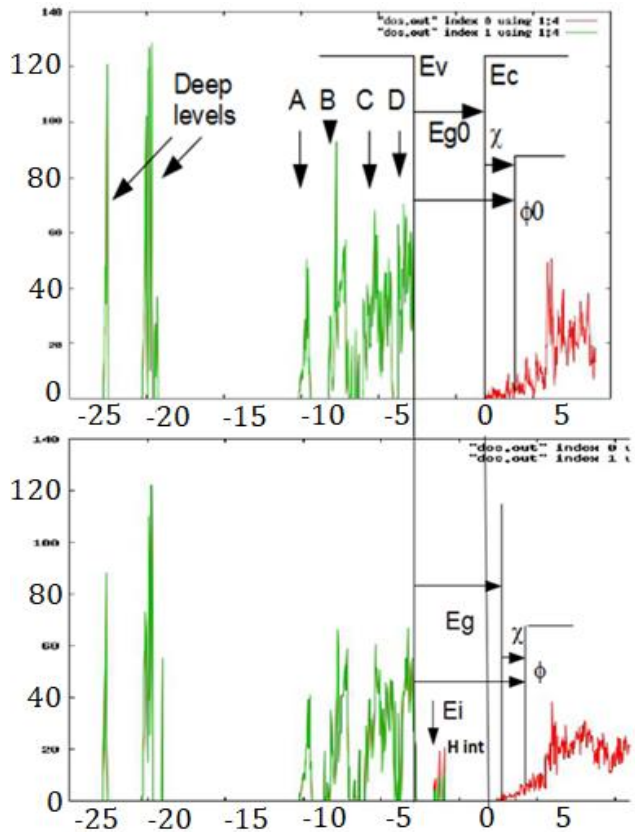
Fig. 2.5. DOS for defectless HAp hexagonal structure (upper image) and DOS with one H-interstitial in the OH channel between two OH groups in the HAp hexagonal unit cell (lower image), a local level E_i (H int) is induced in the forbidden zone, which is characterized by energy E_i \approx E_v + (1,20-1,75) \text{ eV} .
