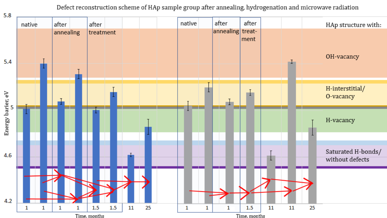
Fig. 3.16. Schemes of defect reconstructions in HAp after annealing, hydrogenation, and microwave irradiation.
