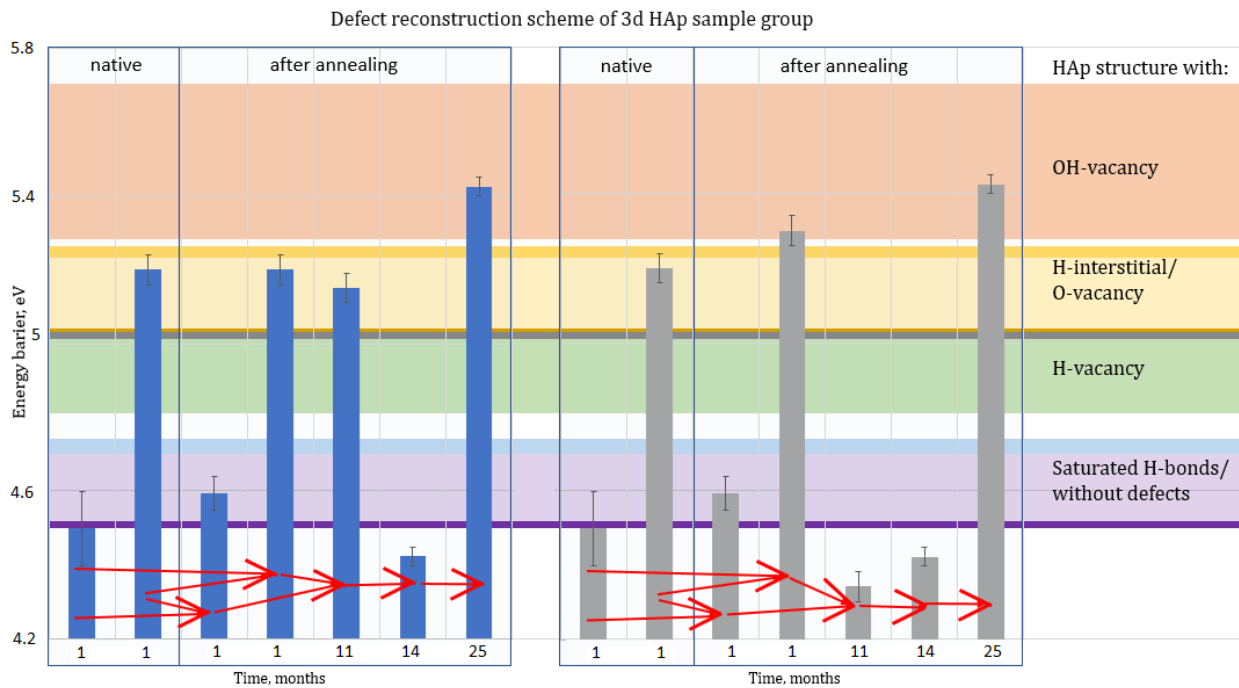
Fig. 3.8. Schemes of defect reconstructions in samples of the Group 3.
