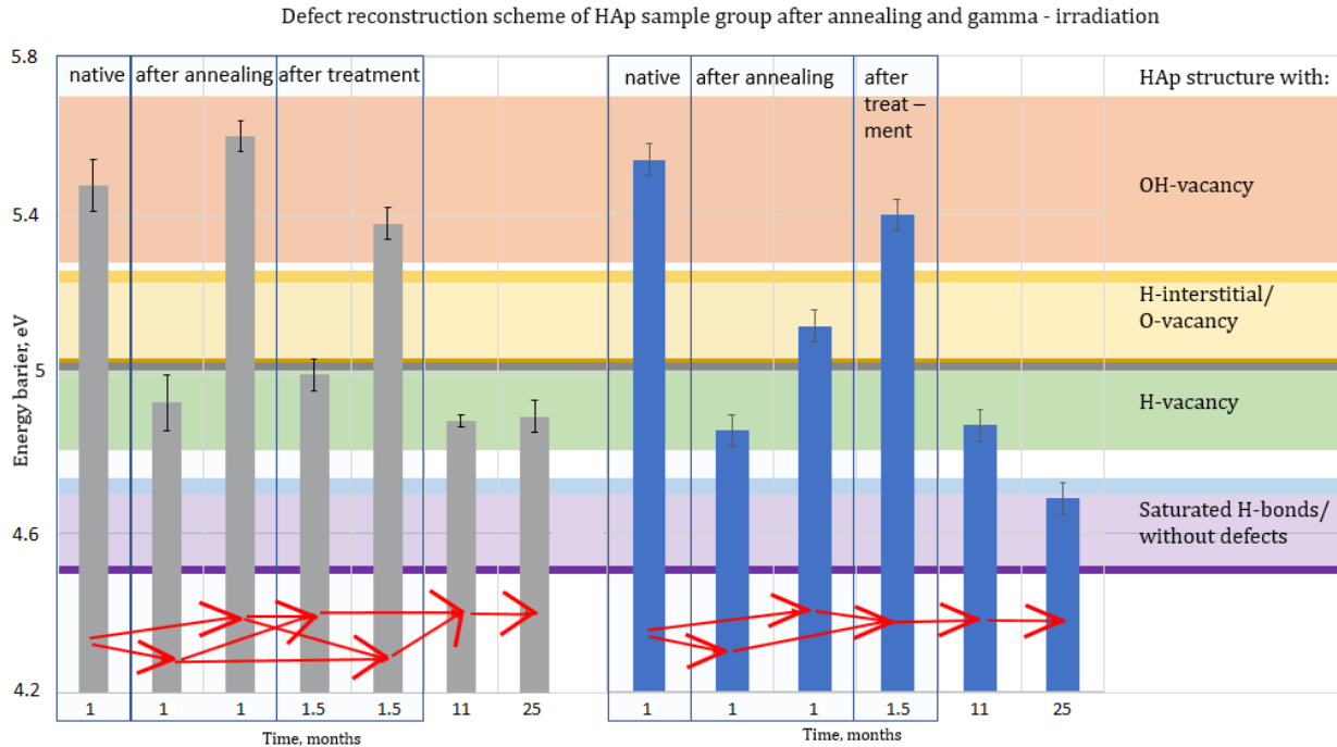
Fig. 3.13. Schemes of defect reconstructions in HAp after annealing and gamma-ray irradiation.
