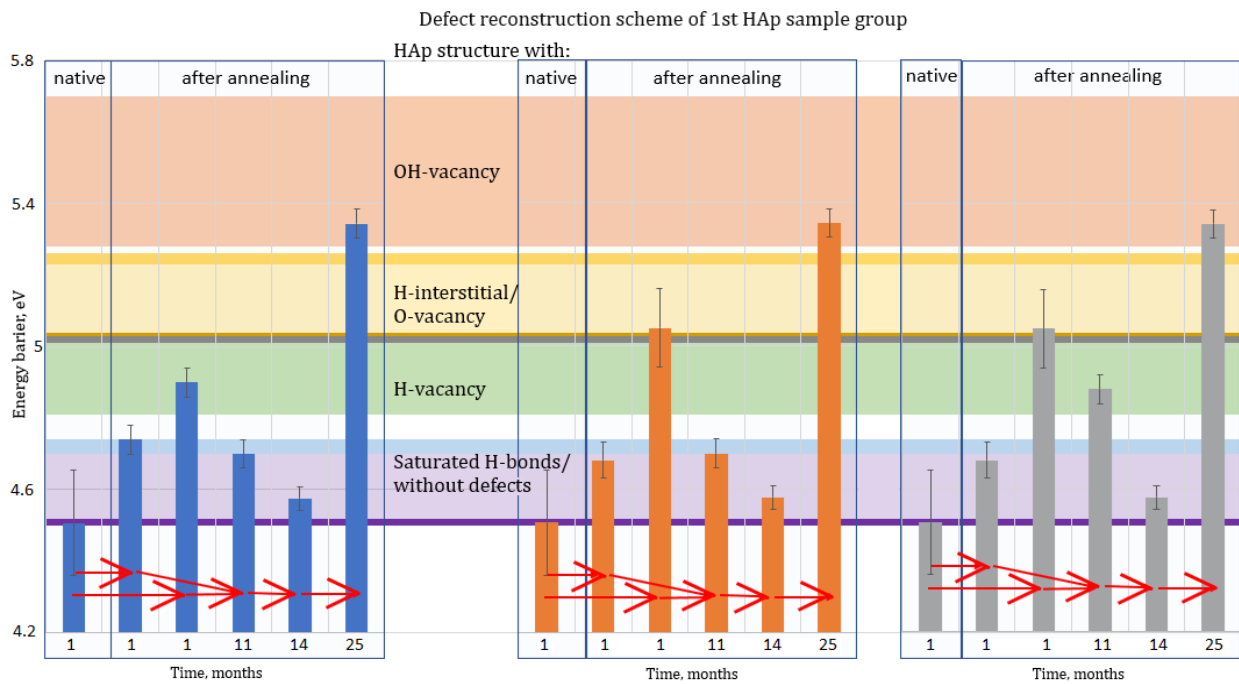
Fig. 3.6. Schemes of the defect reconstructions in samples of Group 1.
