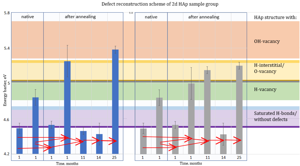
Fig. 3.7. Schemes of defect reconstructions in samples of the Group 2.
