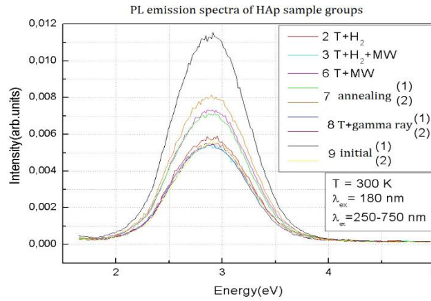
Fig. 3.17. PL emission spectra.
