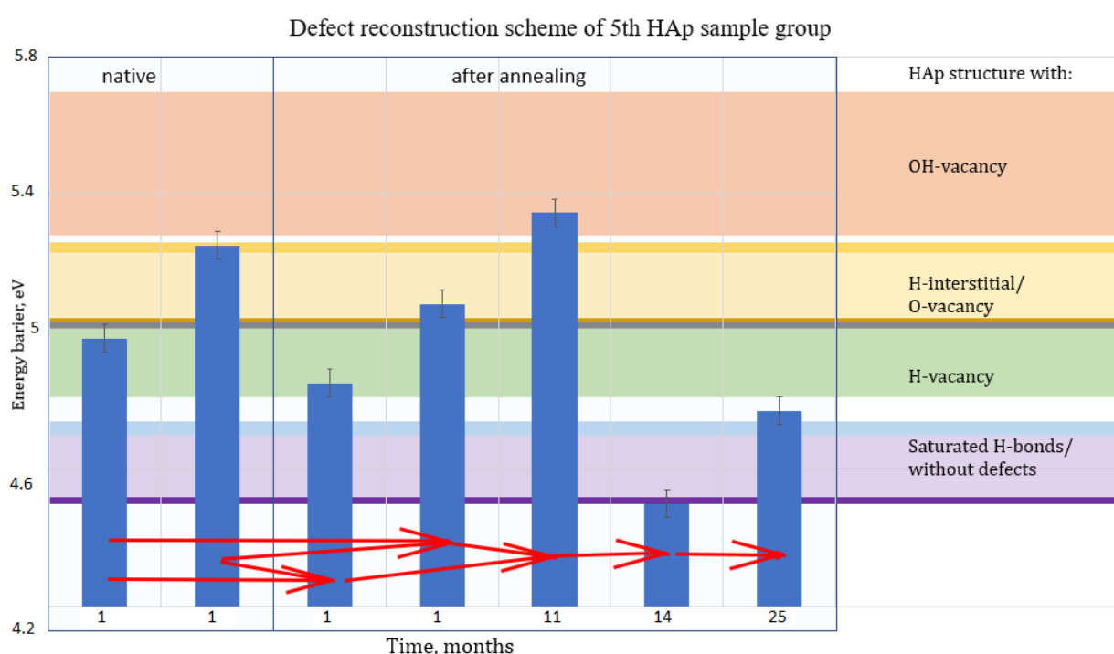
Fig. 3.10. Scheme of defect reconstruction in samples of Group 5.
