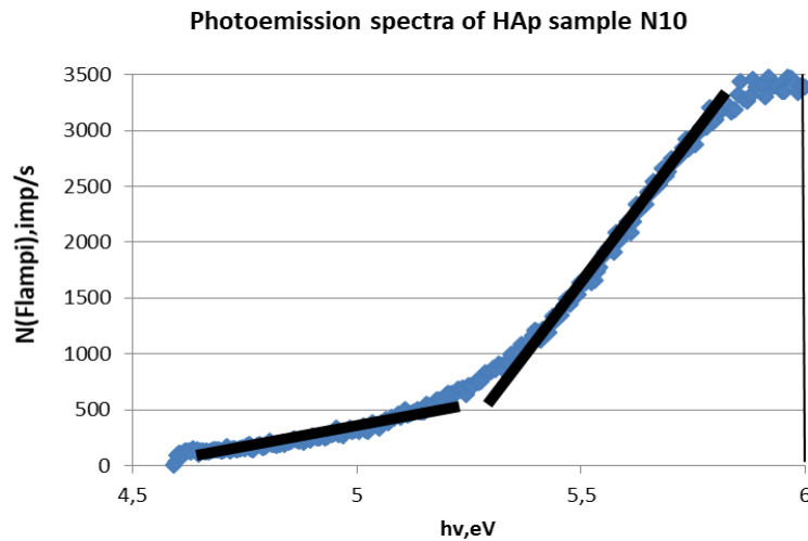
Fig. 3.2. Example of PE spectra of HAp sample with EWF variations, corresponding to two different types of cells with defects.
