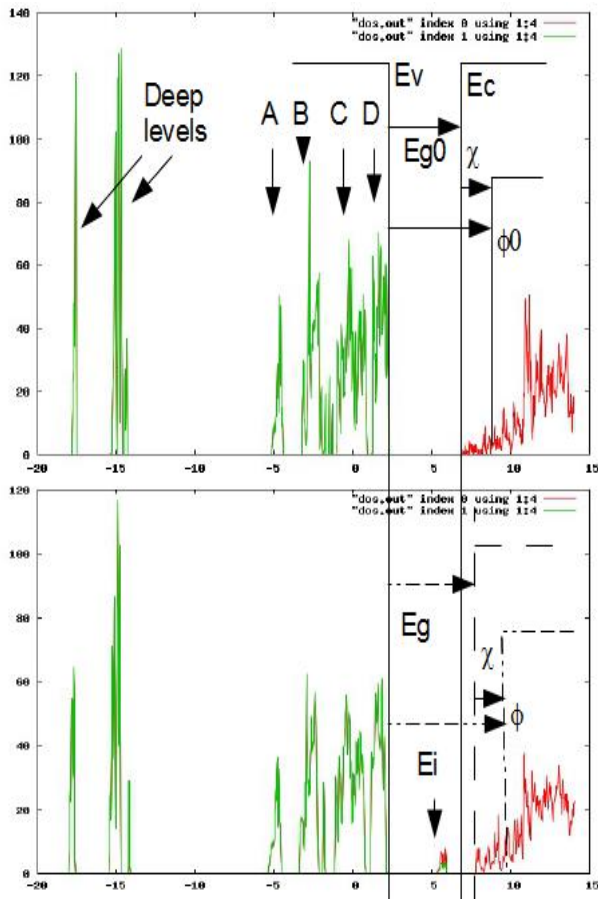
Fig. 2.4. The density of states (DOS) for defectless HAp hexagonal structure (upper image) and HAp with one OH-vacancies per one unit cell (lower image). Here A, B, C & D are the usual levels for HAp, reported in similar works [28, 45].
