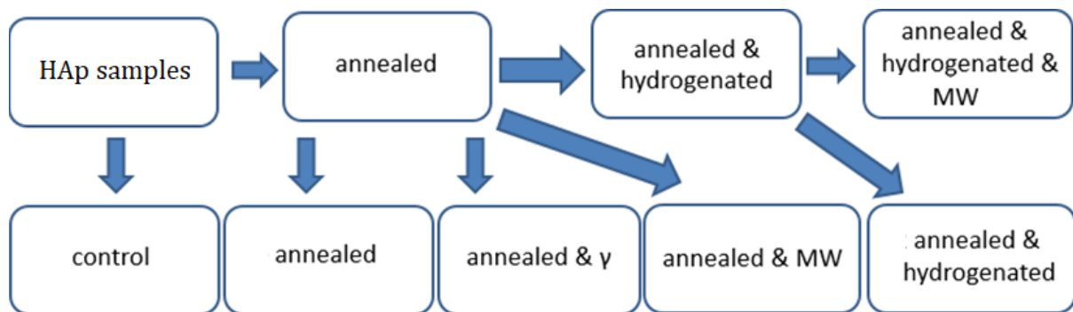
Fig. 3.1. Scheme of applied treatments on HAp samples.
