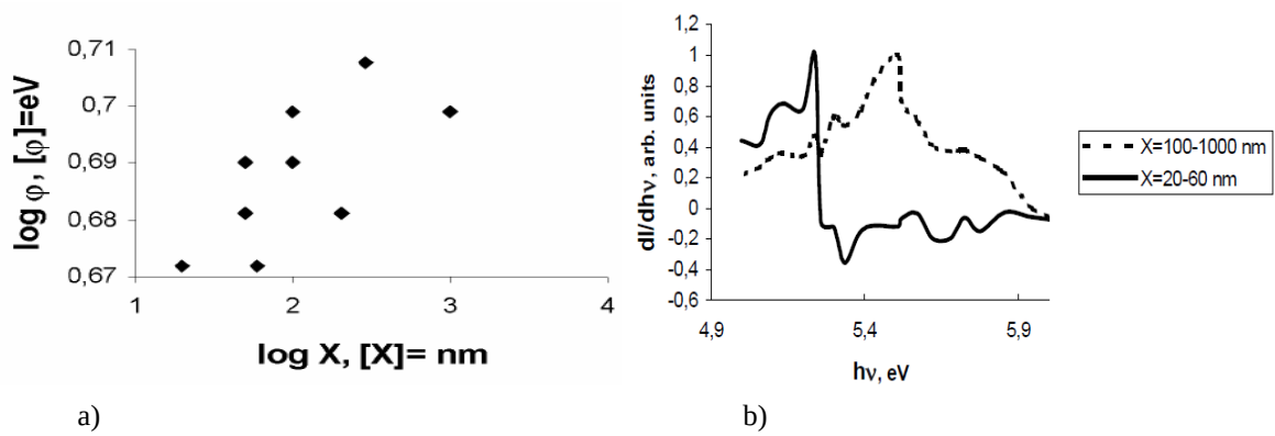
Fig. 2.2. a) Increment of EWF value with increase of HAp NPs size [13, 49]; b) shift of the PE emission peak with the rise of HAp NPs size.
