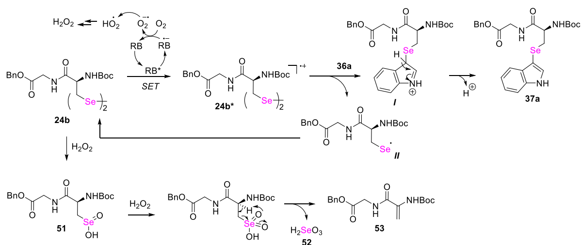
Scheme 20. Proposed mechanism of visible light mediated reaction.
