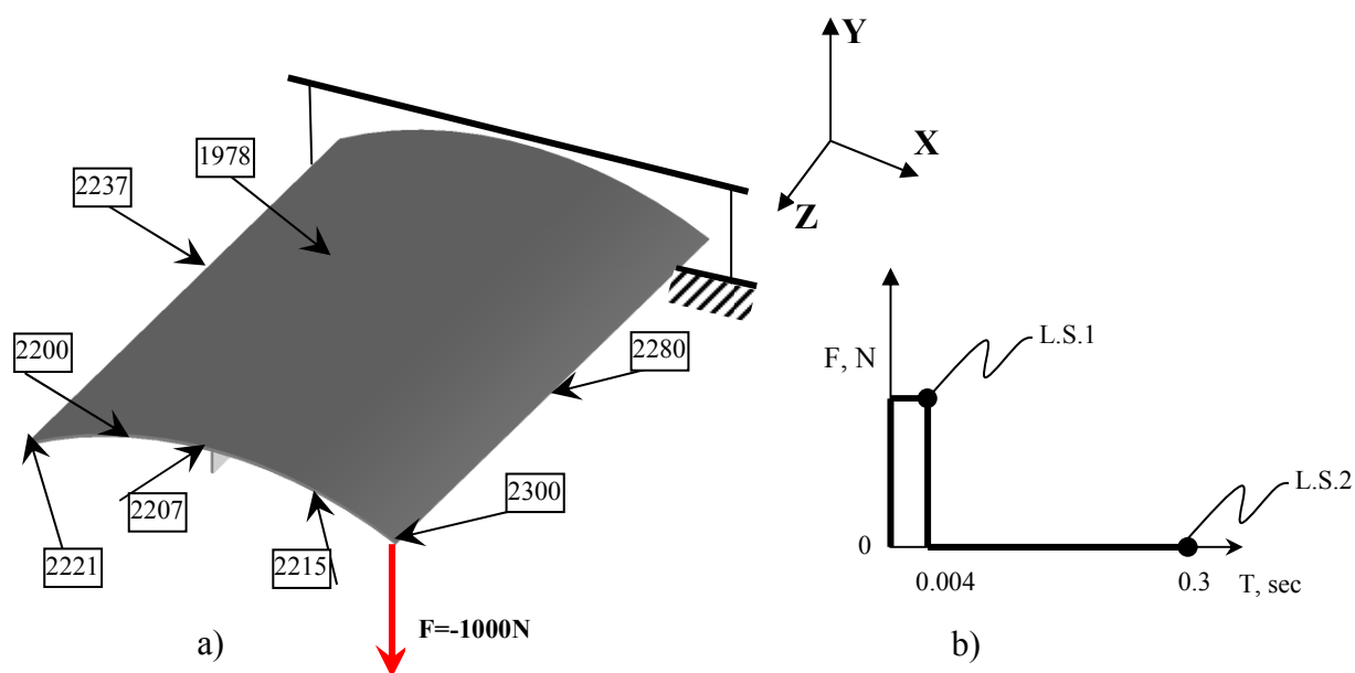
Figure 1. a) covering element – plate with checkpoints, (0.4x0.25x0.002 s-0.015), b) stepped history of loading
