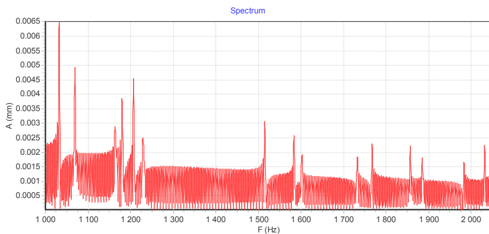
Figure 16. Frequency spectrum for 1000-2100 Hz - synthesis
