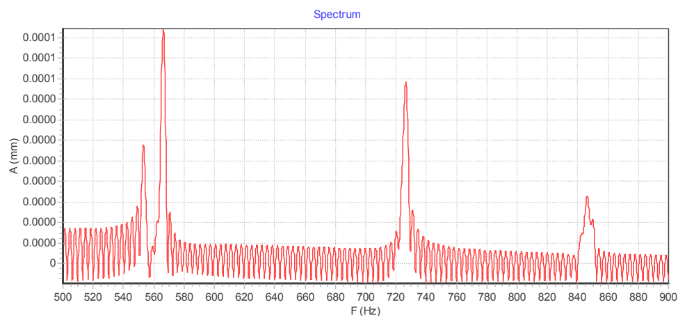
Figure 7. Frequency spectrum in the range 500 – 900 Hz
