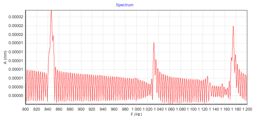
Figure 18. Frequency spectrum 800-1200 Hz of calculated process, 2000 steps
