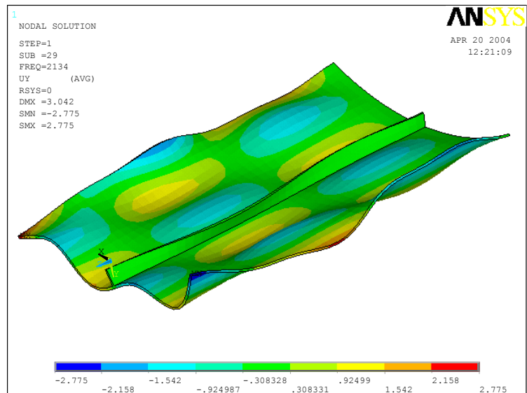
Figure 3. State of strain of a plate along axis Y on 29-th frequency (Table 1), is turned
