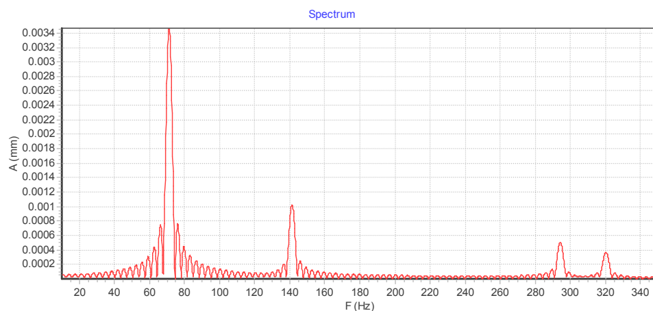
Figure 6. Frequency spectrum in the range 10 – 350 Hz
