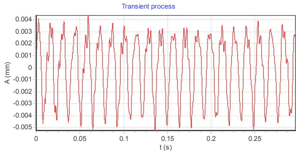
Figure 4. Calculation by ANSYS – displacement of the point №1978 at time along Y-axis (Fig.1.)
