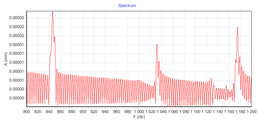
Figure 19. Frequency spectrum 800-1200 Hz of calculated process, 3000 steps
