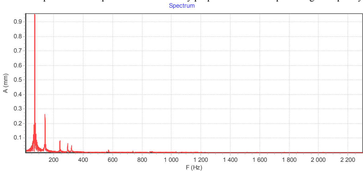
Figure 13. Frequency spectrum 10-2300 Hz of the process synthesized by Polyharmonic program.
