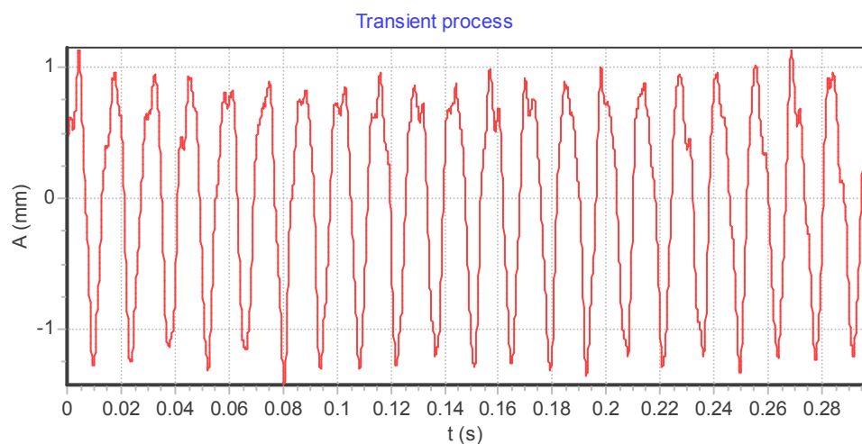
Figure 11. Synthesized displacement process of u vs.time t – amplitude A=1/w^2
