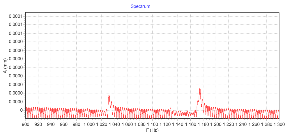
Figure 8. Frequency spectrum in the range 900 – 1300 Hz
