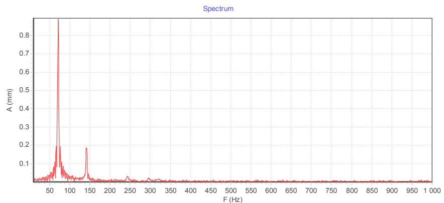
Figure 17. Frequency spectrum 10-2000 Hz – synthesis. Noise level- 20% Dissipation coefficient - 0.000006
