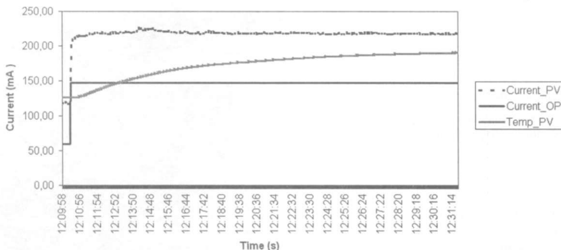
Fig. 2. Experimental graphs of temperature dependence of the motor current: “Current_PV” – current motor winding; “Current_OP” - impact direct of the controller; “Temp_PV” - motor temperature
